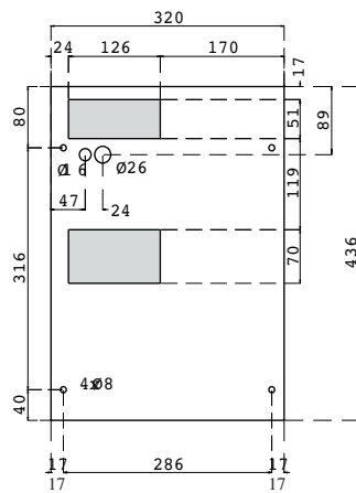
EVE03
