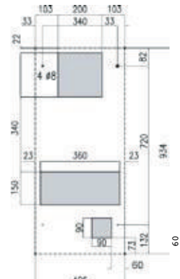
EVE11/20 EVE09/14
