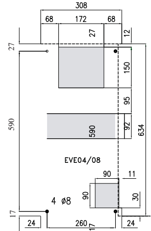
EVE04 EVE08
