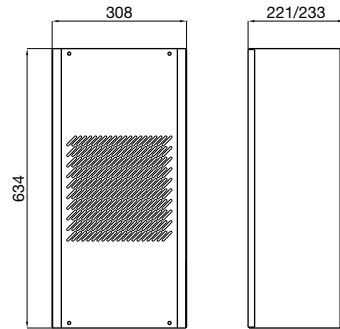
EVE04 EVE08
