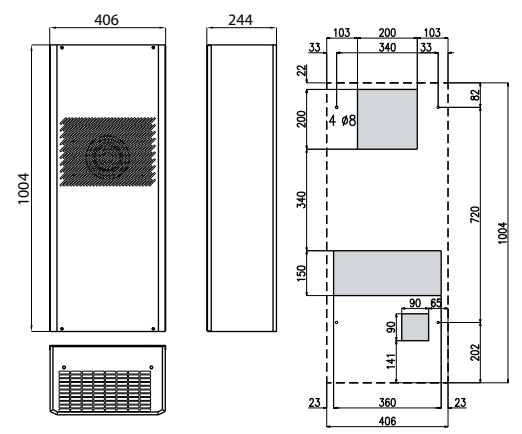
EVE20U
