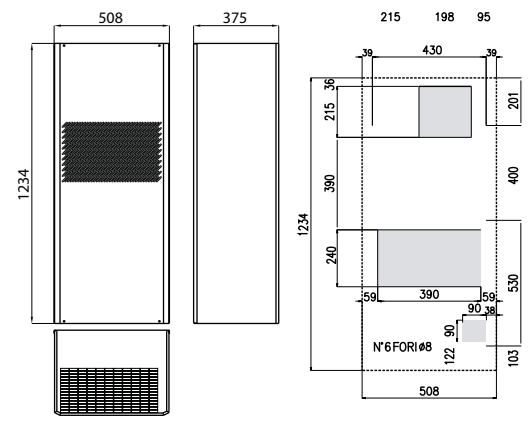
EVE28/EVE41
