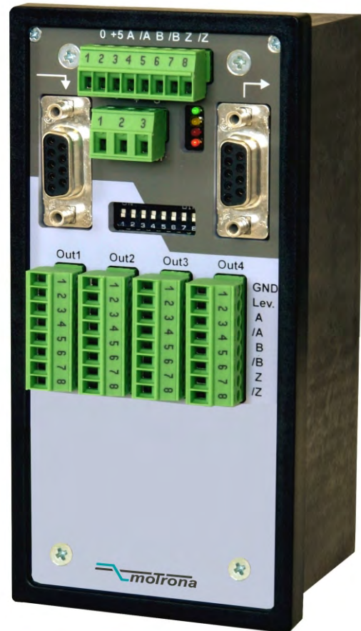
GV 481: Splitter with 4 Output Channels
